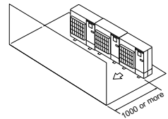
(1) Obstacle at front (open at back, sides and top)
