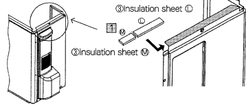
(Top view of Electric box)
